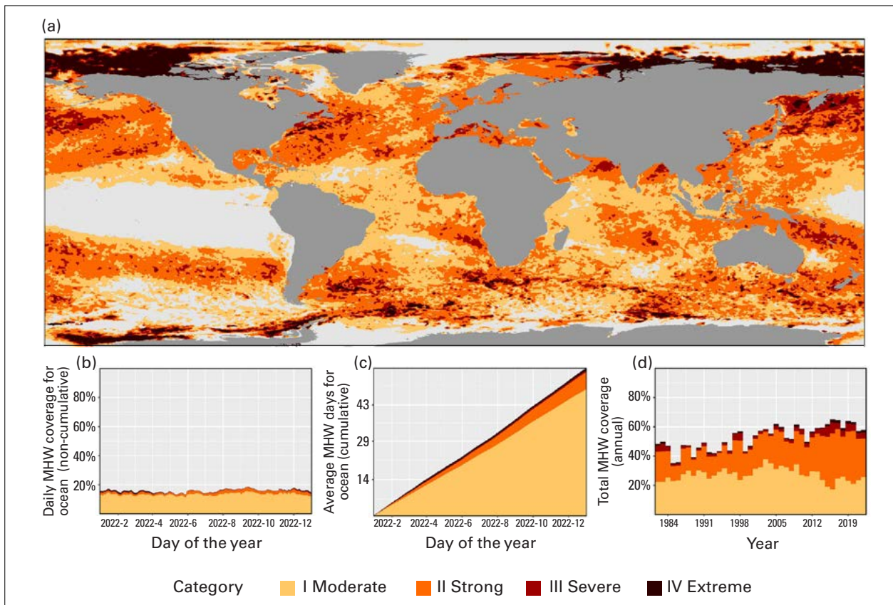
Figure 9. (a) Global map showing the highest MHW category (for definitions, see Data sets and methods ) experienced at each pixel (resolution is 0.25° x 0.25°) over 2022 (reference period 1982–2011). Light grey indicates that no MHW occurred in a pixel over the entire year. (b) Stacked bar plot showing the percentage of the surface of the ocean experiencing an MHW on any given day of the year. (c) Stacked bar plot showing the cumulative number of MHW days averaged over the surface of the ocean. Note: The average is calculated by dividing the cumulative sum of MHW days per pixel weighted by the surface area of those pixels. (d) The annual total surface area of the ocean that experienced a MHW from 1982 to 2022. Data are from the National Oceanic and Atmospheric Administration Optimum Interpolation Sea Surface Temperature (NOAA) OISST.
