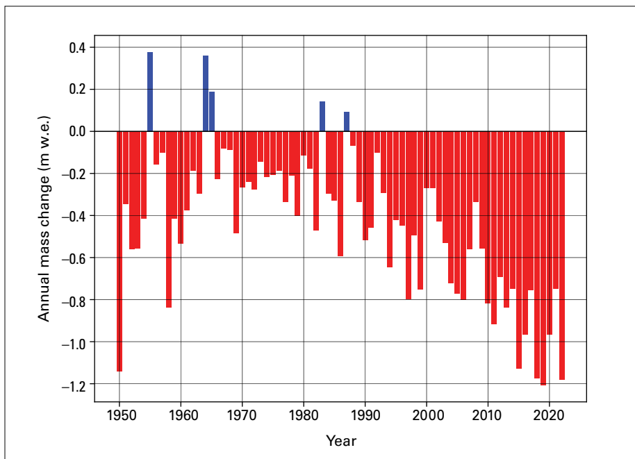
Figure 13. Global annual mass change of a composite of approximately 40 reference glaciers worldwide covering the period 1950–2022.
