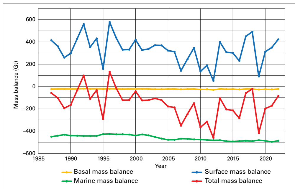
Figure 15. Components of the total mass balance (TMB) of the Greenland ice sheet 1987–2022. Blue: surface mass balance (SMB); green: marine mass balance (MMB); orange: basal mass balance (BMB); red: TMB, the sum of SMB, MMB and BMB.
