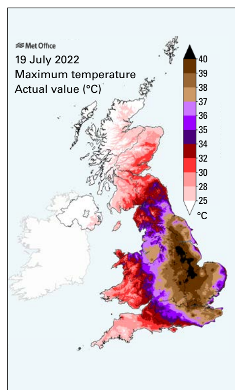
Figure 23. United Kingdom maximum temperatures for 19 July.
